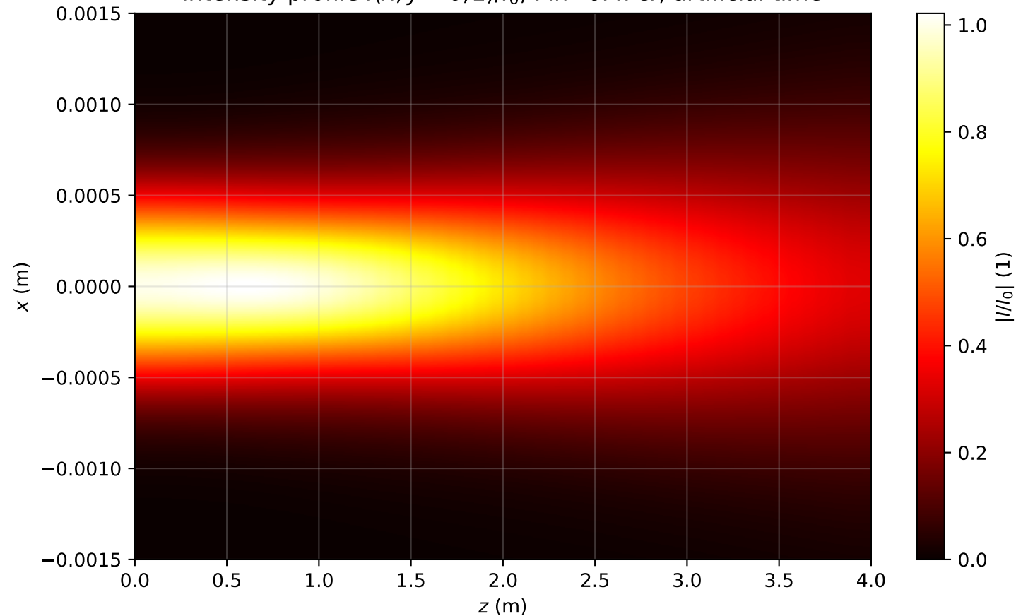
Intensity profile I(x, y = 0, z)/I_0 , P_{in}=0.4P_{cr} , artificial time
